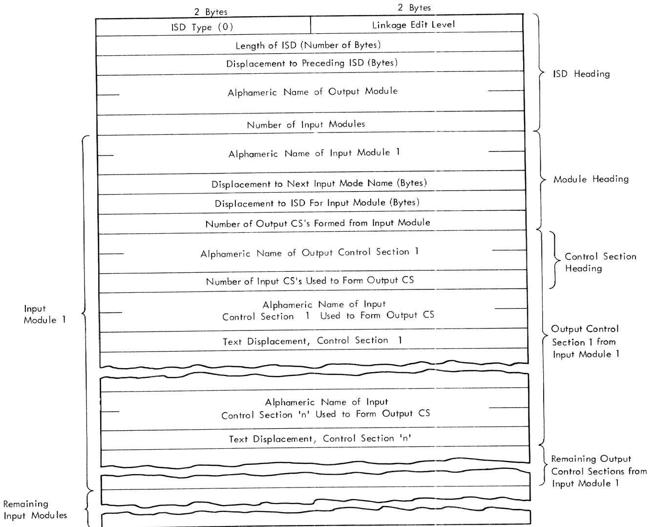
Figure 14. Composite ISD directory format
