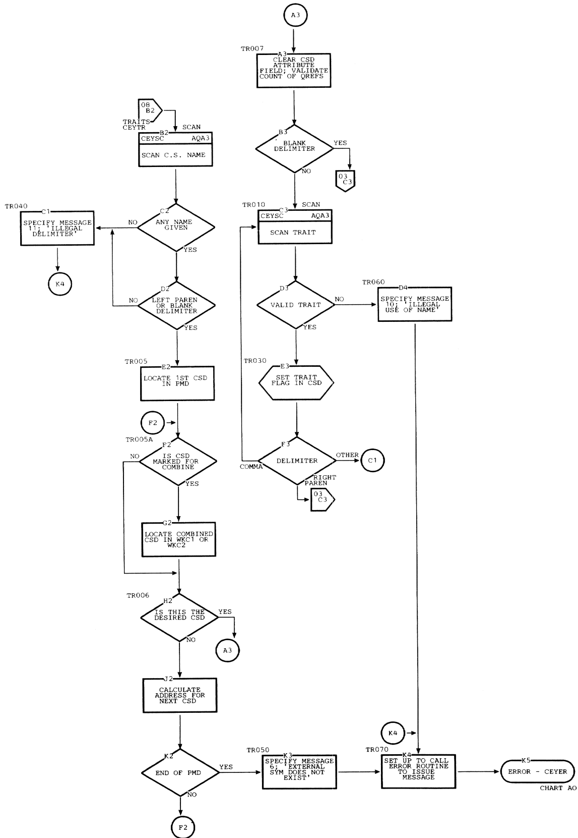
Chart AA. Linkage Editor: TRAITS - TRAITS statement processor (page 8 of 9)
