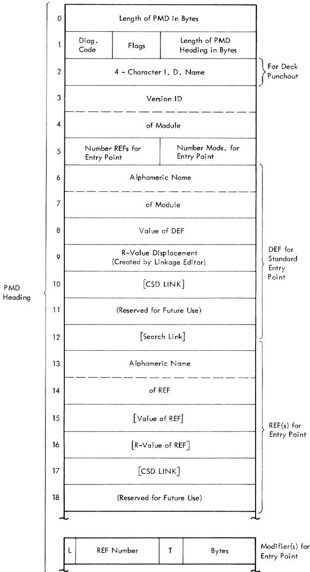
Figure 13. Program module dictionary format (part 1 of 2)
