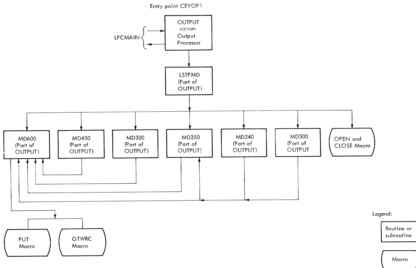
Figure 6. Overview of the output processor
